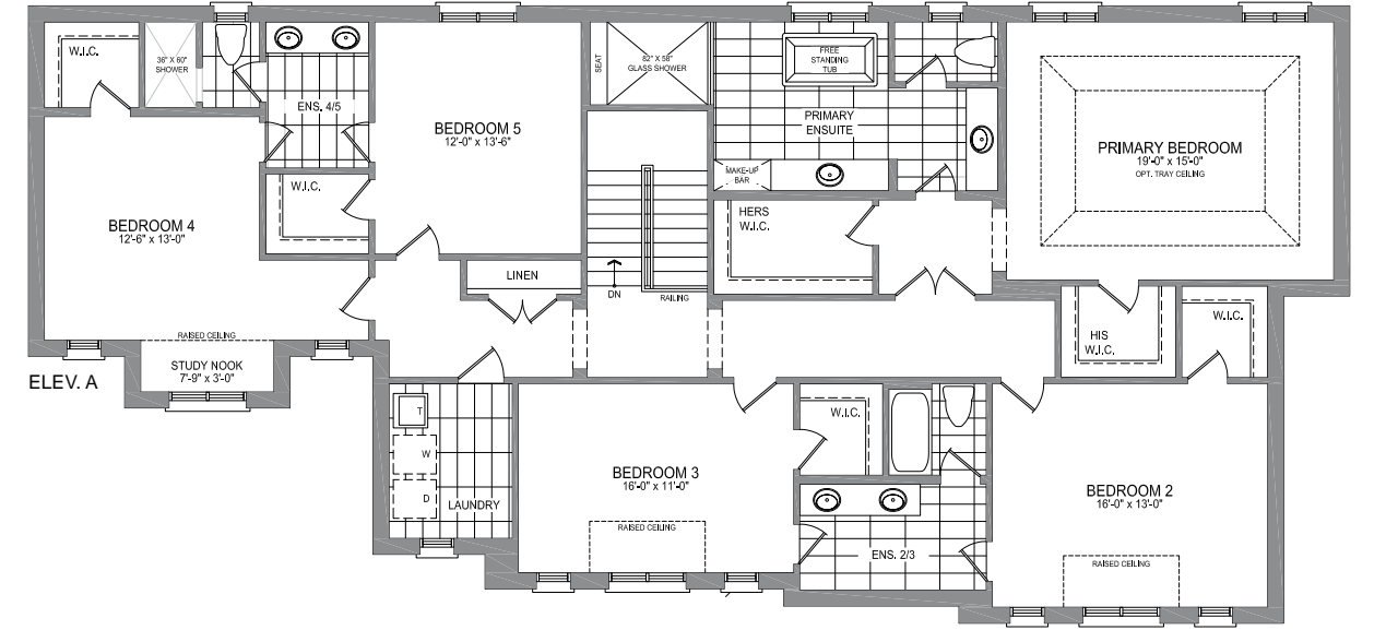
UPPER LEVEL
