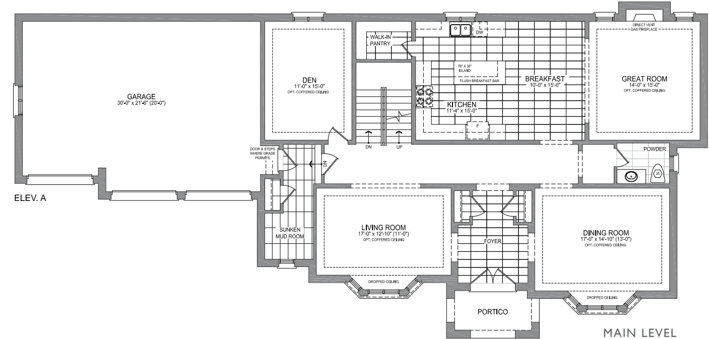
MAIN LEVEL
